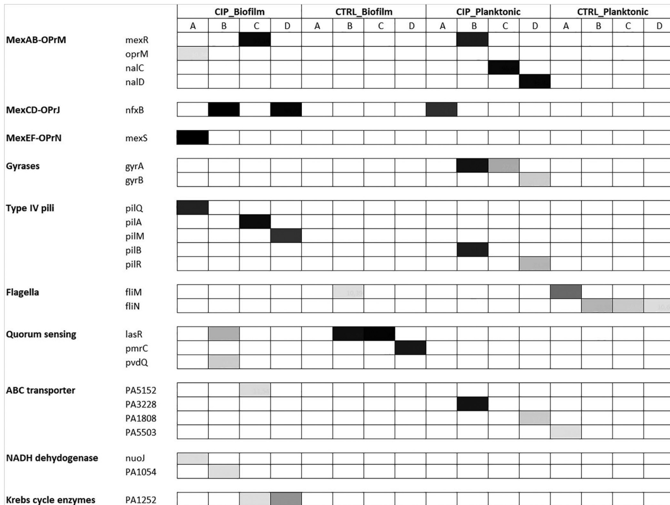
FIG 4 Heatmap showing mutations in CIP and CTRL-evolved populations in both biofilm and planktonic cultures. Genes are clustered according to their function reported in the Pseudomonas Genome Database (26). The intensity of color reflects the frequency of mutations in each replicate population.
